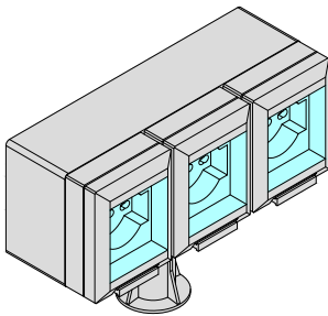
MA90802 3 Prese Schuko 220V-16A 3 SCHUKO 220V-16A SOCKET
