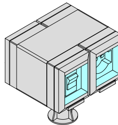
MA90804i 2 Prese Schuko 220V-16A e 2 interruttori magnetotermici 2 Schuko 220V-16A sockets with 2 magnetothermic switches
