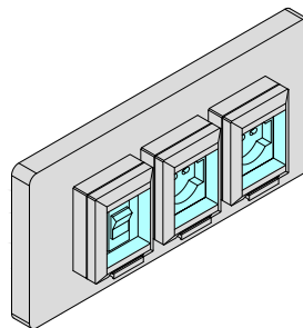
MA90Q213 2 Prese Schuko 220V-16A IP55 1 interrutt. magnetotermico 2 Schuko 220V-16A IP55 sockets with 1 magnetothermal switches
