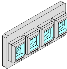
MA90Q211 3 Prese Schuko 220V-16A IP55 interrutt. magnetotermico 3 Schuko 220V-16A IP55 sockets with magnetothermal switch
