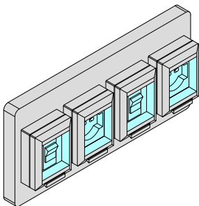
MA90Q212 2 Prese Schuko 220V-16A IP55 2 interruttori magnetotermici 2 Schuko 220V-16A IP55 sockets with 2 magnetothermal switch
