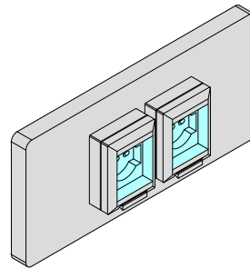
MA90Q220UPS 2 Prese Schuko UPS 220V-16A IP55 2 Schuko UPS 220V-16A IP55 sockets
