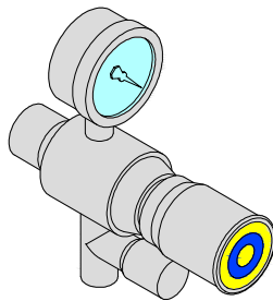
MA90RID Rubinetto gas 1 via con manometro Gas tap, 1 way, with manometer
